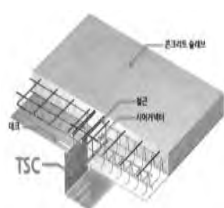
<TSC BEAM>
